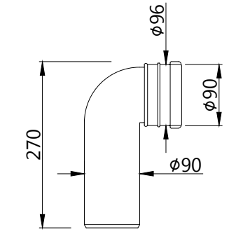
WASTE BEND
